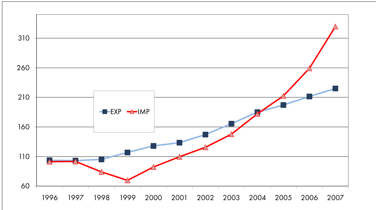
Figure 3: Dynamics of Real Exports and Imports
